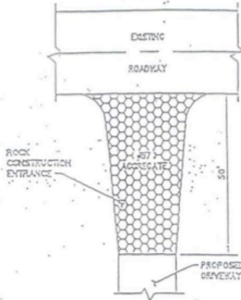
PLAN VIEW
