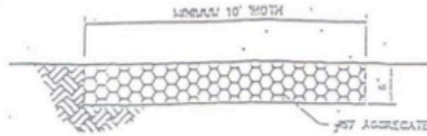
ELEVATION VIEW
